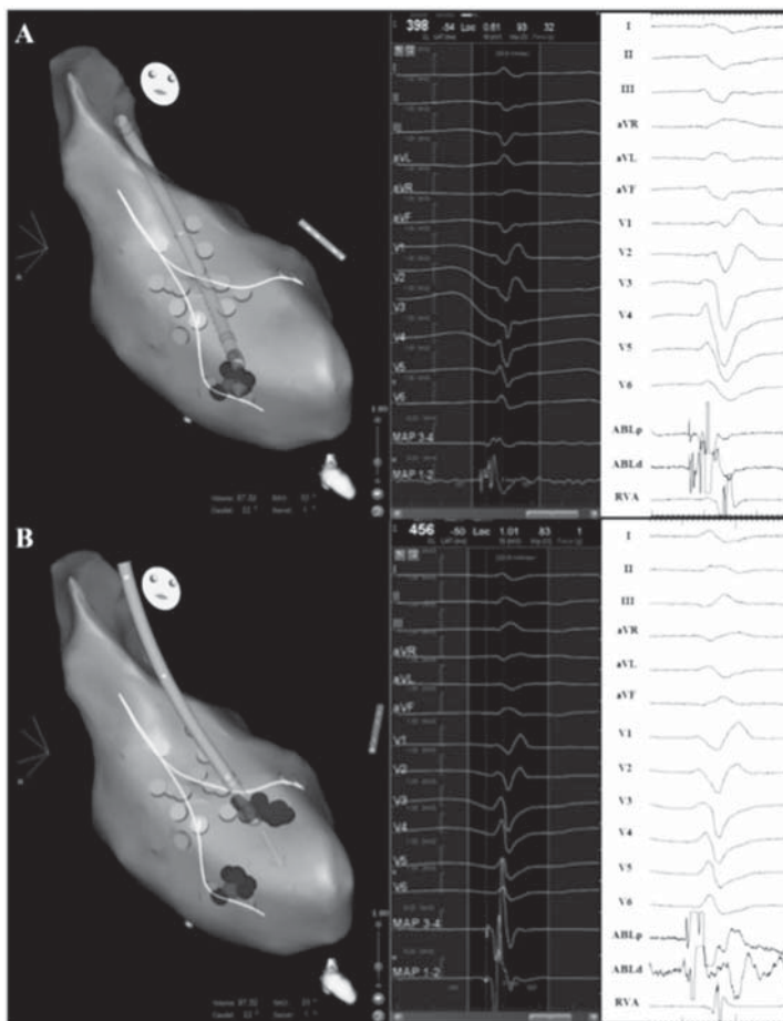
Fig. 3. Three-dimensional electro-anatomical maps using CARTO3 system (Biosense Webster, CA, USA) showing the LV septum with a 22° caudal 33° right anterior oblique view. The His Bundle separating into the anterior and posterior fascicle are roughly tracked in yellow (lines and dots) according to the intracardiac recordings using the ablation catheter. Red dots indicate the sites of RF delivery. Twelve lead ECG (200 mm/s) with the potentials recorded at the ablation sites are shown on the right. Top panel shows the ablation of the first PVC morphology, whereas bottom panel indicates the ablation of the second one. In both cases, at the ablation sites, the local ventricular near field is clearly preceded by a discrete high-frequency potential, i.e. Purkinje potential (ablation catheter distal and proximal electrodes). The recording of such potentials is fundamental for the effective ablation in these cases.
